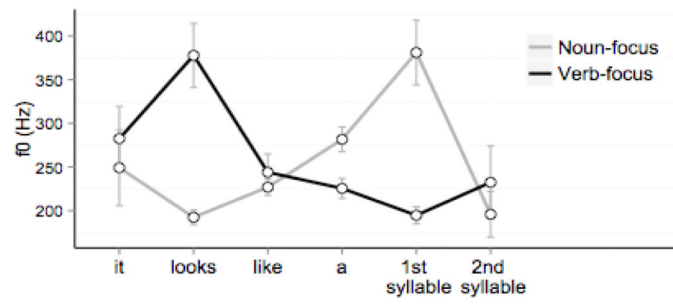
Figure 2. Mean syllable duration (a) and F0 (b) in the Verb-focus and Noun-focus conditions.
